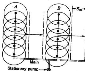
Fig .2 Fully portable sprinkler irrigation system
